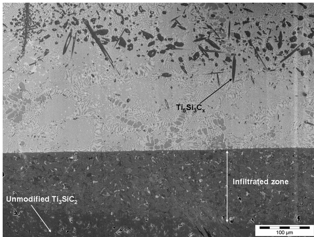
Fig. 4: SEM micrograph representing a cross-section of the interface between an AgCu-2,5wt.%Ti melt and a Ti_3SiC_2 substrate after 7 min of contact at 800°C and 10 min at 900°C (experiment presented by open triangles in Figure 2)
