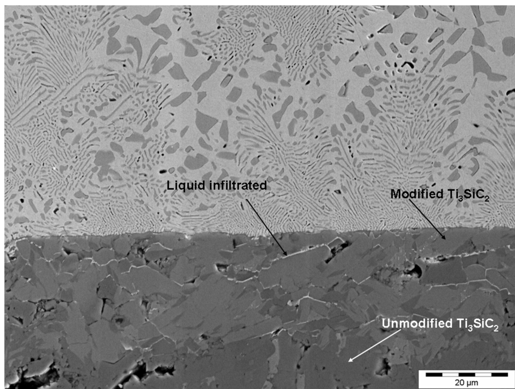
Fig. 3: SEM micrograph representing a cross-section of the interface between an AgCu eutectic and a \text{Ti}_3\text{SiC}_2 substrate after a prior heat treatment of the substrate at 900^\circ\text{C} and a subsequent contact time of 420 s at 800^\circ\text{C} (filled square in Figure 1).
