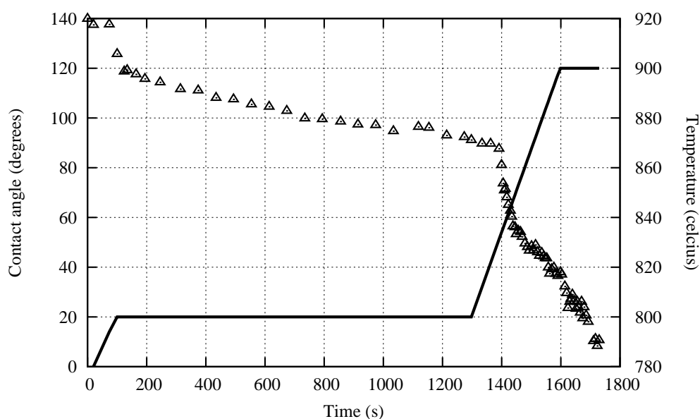
Fig. 2: Contact angle measured by the classical sessile drop technique as a function of time for AgCu-2,5wt.%Ti alloy on \text{Ti}_3\text{SiC}_2 at 800^\circ\text{C} during about 1300 s and then after heating up to 900^\circ\text{C}
