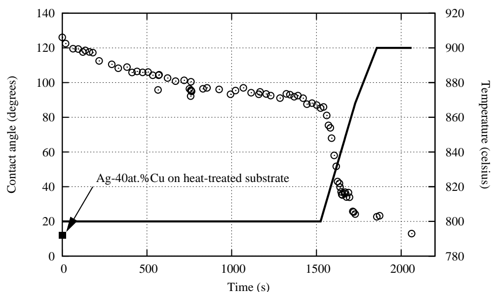
Fig. 1: variations in contact angle, \theta , and temperature as functions of time for the spreading of two AgCu eutectic droplets over \text{Ti}_3\text{SiC}_2 in the experiments performed by the dispensed drop technique: (i) at 800°C after pre-heating of the substrate at 900°C (filled square, indicated by the arrow), (ii) at 800°C during about 1500 s then heated up to 900°C (open circles). Temperature vs. Time is presented by solid line.
