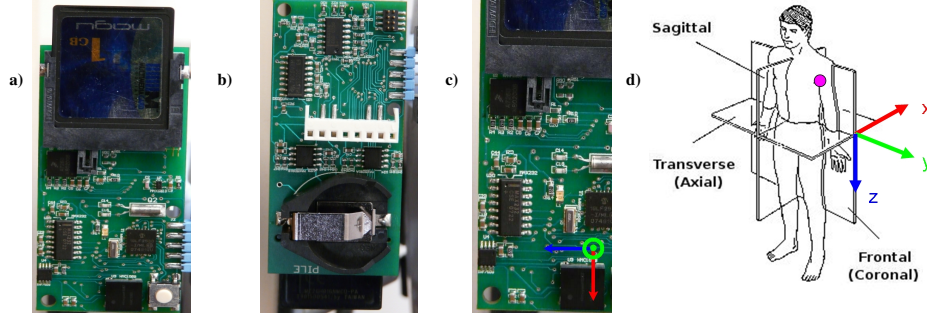
Figure 1: ACTIM6D and its positioning on the subject. (a): front side of the circuit board, (b): back side of the circuit board, (c): Positioning of the subject basis on the circuit board, (d): Positioning of the subject basis
