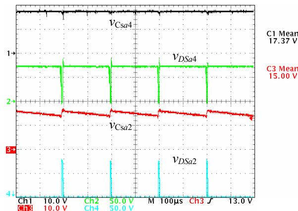
Fig. 10: Experimental results for v_{Csa2} , v_{Csa4} , v_{DSa2} , and v_{DSa4} in the same conditions as in Fig. 9 and m = 0.95 .
