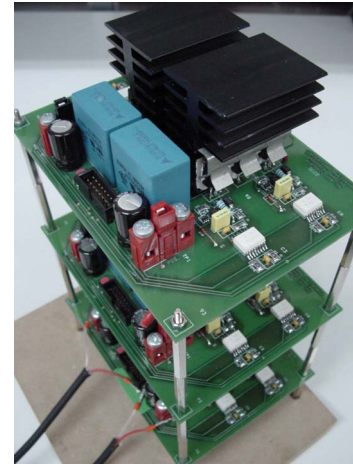
Fig. 5: Three-level three-leg dc-ac converter. (a) Topology. (b) Prototype using 150 V MOSFETs as devices S_{xi} .
