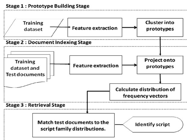
Figure 2. Block diagram of script identification.
