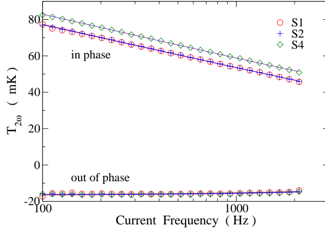
FIG. 1: (Color online) Typical in-phase and out-of-phase temperature oscillations of the heater/thermometer line, versus current frequency. Input power: 3 \text{ W.m}^{-1} . Symbols: experimental points. Lines: fits using eq.(1).
