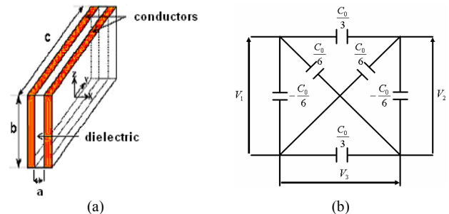
Fig.13. Equivalent circuit for inter-layer capacitances
