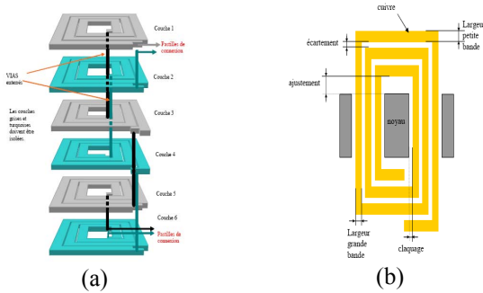
Fig.17. Geometry of studied LCT planar primary layers
