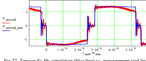
Fig.27. Tension Sa-Sb: simulation (blue line) vs. measurement (red line)
