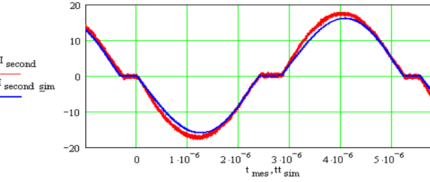
Fig.28. Current at secondary of LCT: simulation (blue line) vs. measurement (red line)
