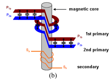
Fig. 1. Principle of LCT components
