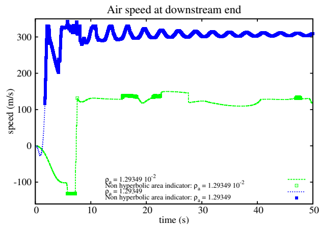
FIGURE 9. Non constant upstream boundary conditions: numerical results at downstream end
