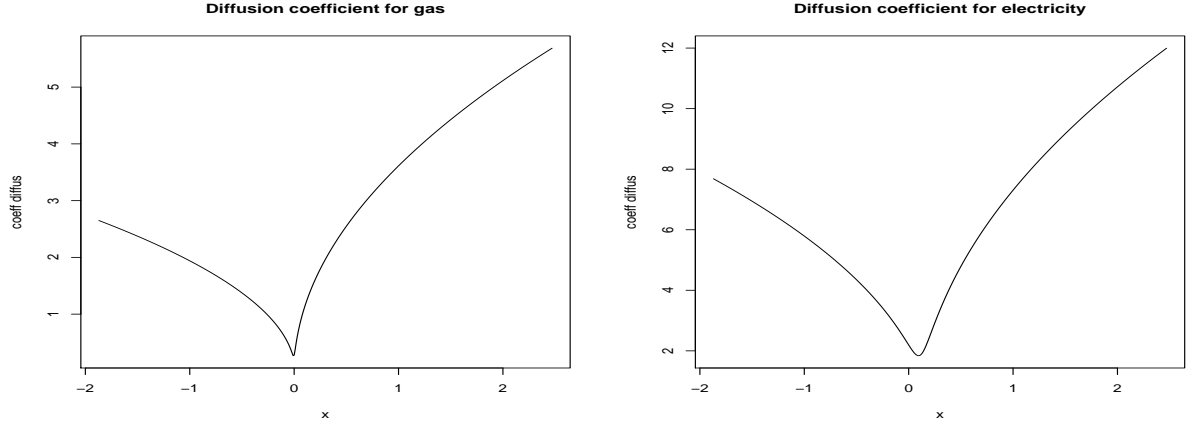
Figure 6: Squared diffusion coefficients using fitted parameters \alpha_g = 2.5 , \beta_g = 1.4 , \delta_g = 0.01 , l_g = -0.0019 and \alpha_e = 3.5 , \beta_e = 1.2 , \delta_e = 0.08 , l_e = 0.11 .
