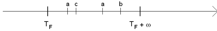
Fig. 1. A sequence S of events from E = \{a, b, c\} and its window F of size \omega beginning at T_F .
