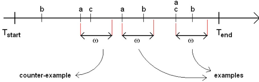
Fig. 2. Among the 3 windows of size \omega beginning on events a , one can find 2 examples and 1 counter-example of the rule a \xrightarrow{\omega} b .
