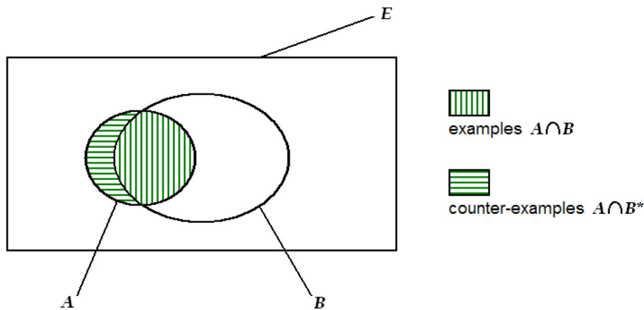
Figure 1. Venn diagram for the rule a \rightarrow b .
