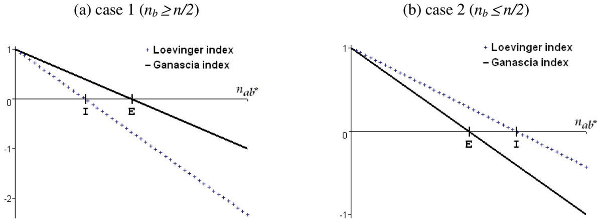
Figure 3. Comparison of Ganascia and Loevinger indexes. ( E : equilibrium, I : independence)
