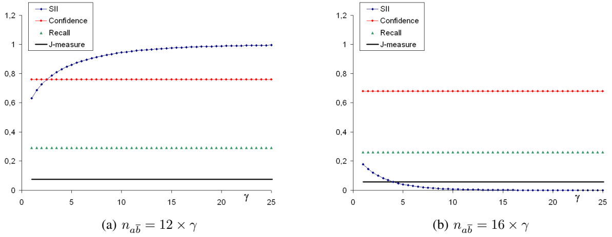
Fig. 7. SII , confidence, recall, and J-measure with sequence repetition. ( n_a = 50 \times \gamma , n_b = 130 \times \gamma , \omega = 10 , L = 1000 \times \gamma )
