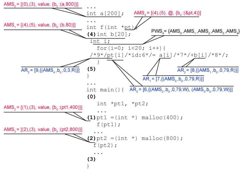
Fig. 4. Abstraction example.
