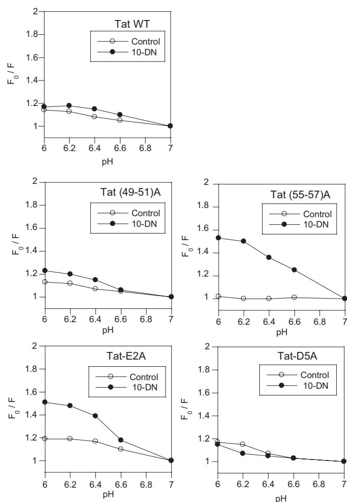
FIGURE 9. Insertion of Tat mutants into lipid vesicles at mildly acidic pH. Tat or the indicated mutant (2 \mu\text{M} ) was added to lipid vesicles composed of PC/PG (Control) or PC/PG/10-DN (10-DN) in citrate buffer. F_0/F is the ratio of fluorescence intensity at pH 7.0 relative to that at the indicated pH. Representative results of triplicate experiments are shown. WT, wild type.
