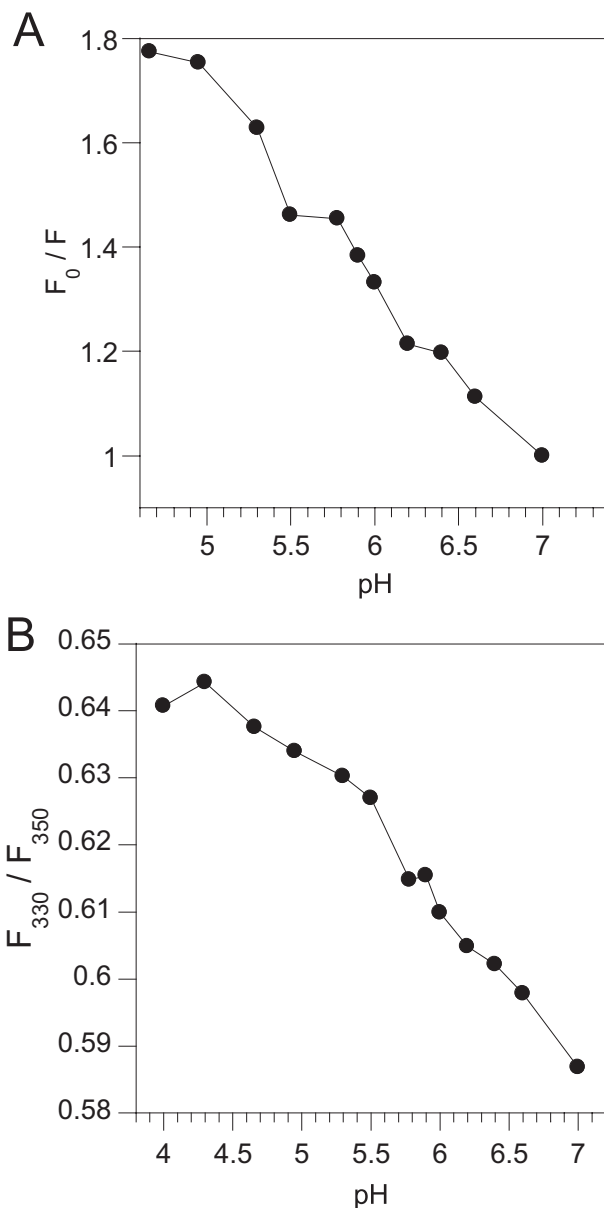
FIGURE 1. Effect of pH on the Trp fluorescence of Tat in the absence of membrane. A, fluorescence decreases upon acidification. Samples contained 2 \mu\text{M} Tat in 150 mM NaCl, 50 mM citrate (citrate buffer) at the indicated pH. F_0/F is the ratio of fluorescence intensity at pH 7.0 relative to that at the indicated pH. B, emission maximum shift as monitored by the ratio of fluorescence intensity at 330 nm to that at 350 nm. The increase in this ratio as the pH dropped denotes a blue shift. Representative results of triplicate experiments are shown.
