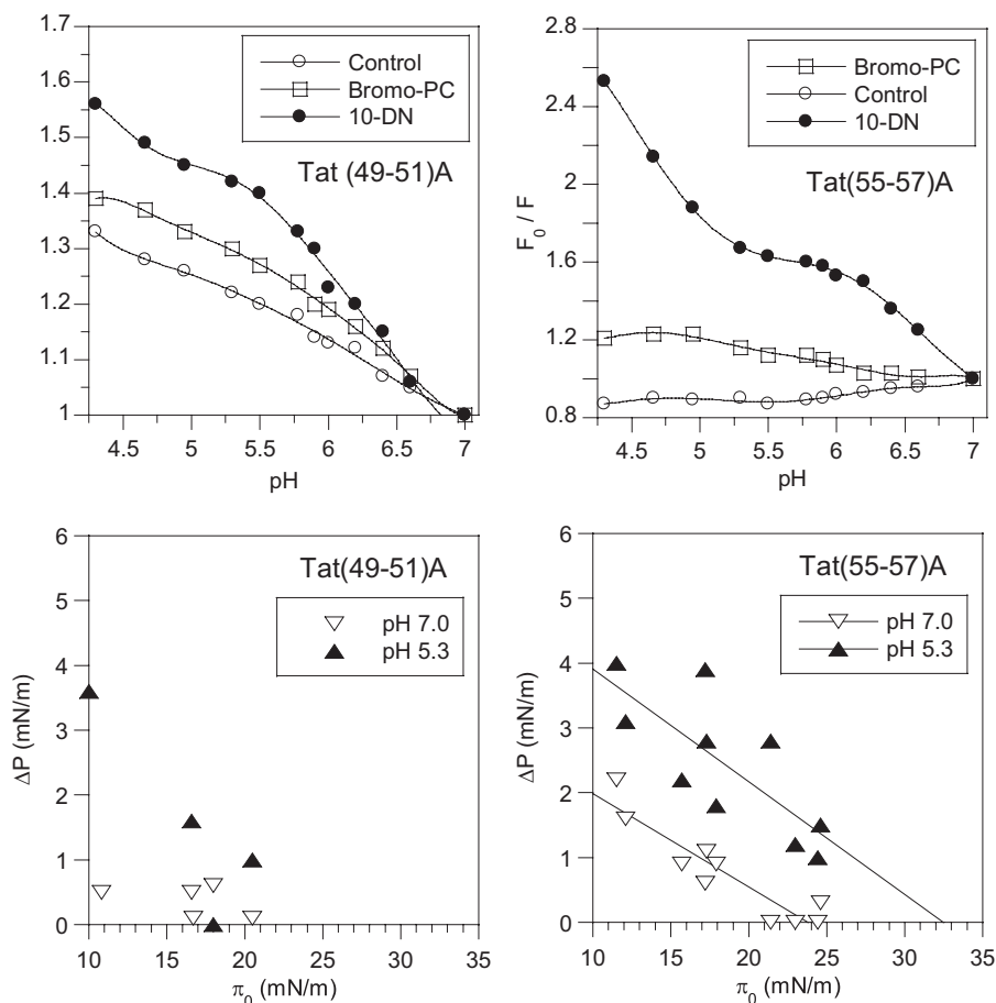
FIGURE 8. Membrane insertion of Tat basic domain mutants. Upper panels, quenching of mutant Trp fluorescence by lipid vesicles. Lower panels, monolayer penetration of Tat basic domain mutants. Experiments were performed as described in the legend to Fig. 3. The statistical significance of the linear regressions is p < 0.01 for Tat(55-57)A at pH 5.3 and p < 0.001 at pH 7.0.
