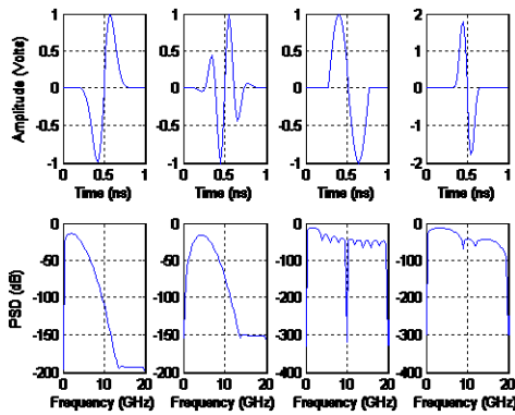
Fig 4. UWB pulse waveform.
