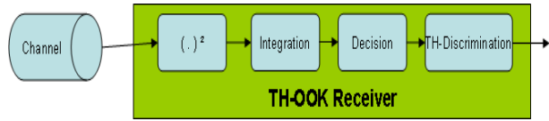
Fig. 20. TH-OOK non coherent receiver architecture.
