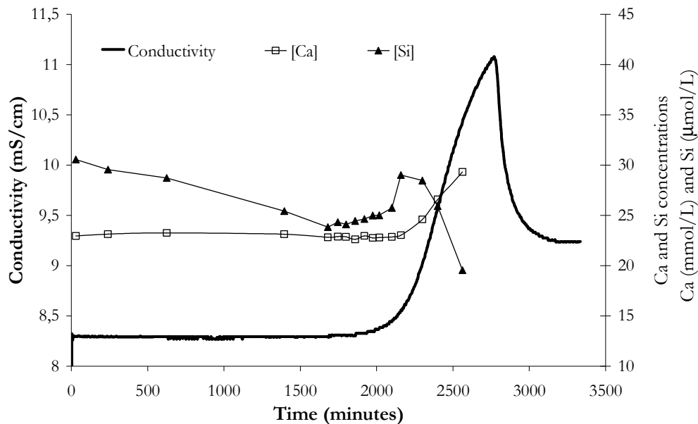
Figure 8: Silica and calcium concentrations evolution and conductimetric curve obtained during C_3S hydration in a lime saturated solution ( L/S=250 ) in presence of 5% of latex with respect to the C_3S .
