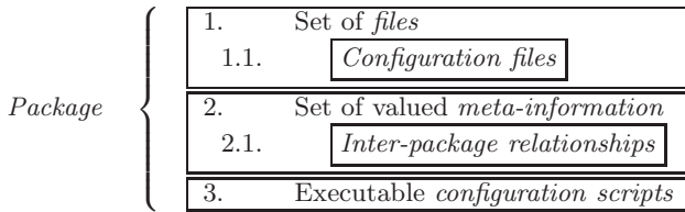
Figure 1: Constituents of a package.
