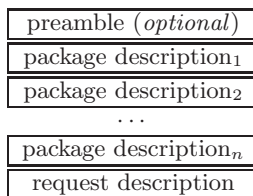
Figure 2: Overall structure of a CUDF document.
