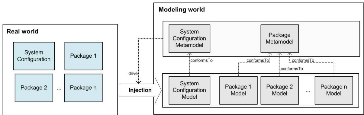
Figure 2: Model injection
