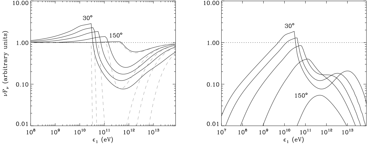
Fig. 3. Spectra as seen by an observer at infinity, taking into account the effect of cascading. Calculations are applied to LS 5039 at periastron for different viewing angle \psi = 30^\circ, 60^\circ, 90^\circ, 120^\circ and 150^\circ . Left panel: Complete spectra (solid line) are compared to the pure absorbed (light dashed line) and injected (dotted line) spectra. The contribution from the cascade is presented in the right panel .
