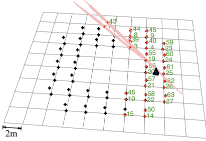
Fig. 5. Simulated 3D environment for 6-DOF monocular SLAM.
