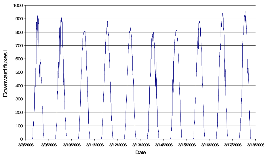
Fig. 5. Downward shortwave fluxes (in \text{W}/\text{m}^2 ) observed at Djougou from pyranometers (Kipp and Konen) measurements for the 8 to 18 March period.
