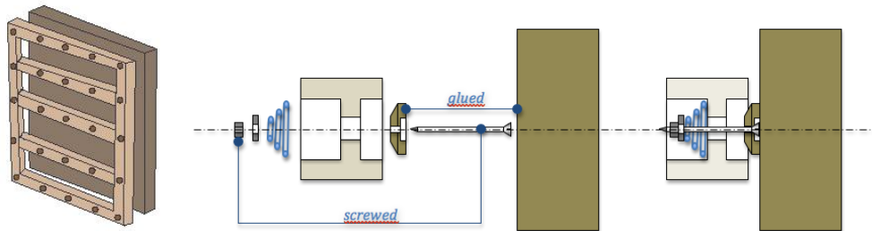
Fig. 1. Back-framing technique
