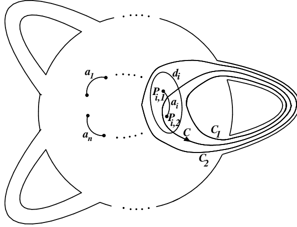
Figure 2: The slide S_{i,C} = T_{C_1}^{-1}T_{C_2}^\varepsilon s_i of the arc a_i along the curve C .
