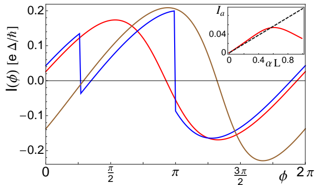
FIG. 2: (Color online) Numerical results for the CPR of a two-level dot with \theta = 0 for b_x = 0.3\Delta , 0.7\Delta and 0.9\Delta (red, blue, brown curves, respectively, with increasing |I_a| ). Parameters: \alpha L = 0.4 , \Gamma_{L,11} = 2\Delta , \Gamma_{L,22} = 0 , \Gamma_{R,11} = \Gamma_{R,22} = \Delta/2 , \epsilon_1 = -\epsilon_2 = 0.65\Delta , L = 25 nm, \Delta = 1 meV, and m = 0.035m_e . Inset: I_a from numerics (red solid curve) and from Eq. (12) (black dashed curve) vs \alpha L , with b_x = 0.5\Delta and same other parameters as in main panel.
