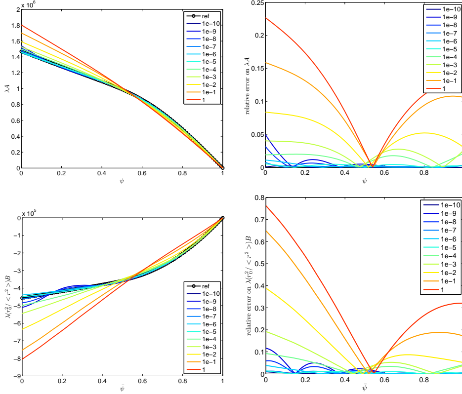
Figure 3. Twin experiment with noise free measurements and different regularization parameters \epsilon ranging from 10^{-10} to 1. Left column: identified functions \lambda A(\bar{\psi}) , \lambda r_0^2 < \frac{j(r, \bar{\psi})}{r^2} > B(\bar{\psi}) for each different \epsilon value, and the known reference functions. Right column: relative errors.
