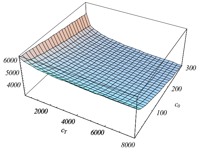
Figure 7 Expected option value (in Euros) of a patent as a function of the initial and final renewal fees
