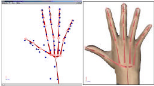
Figure 6. Markers can reshape and animate a generic hand model. Left: Markers (blue dots) can drive a joints/bones structure (red). Right: In the skinning algorithm, the pseudo-bones will influence the vertexes of the textured 3D object.
