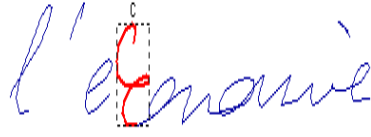
Figure 6. Segmentation error.
