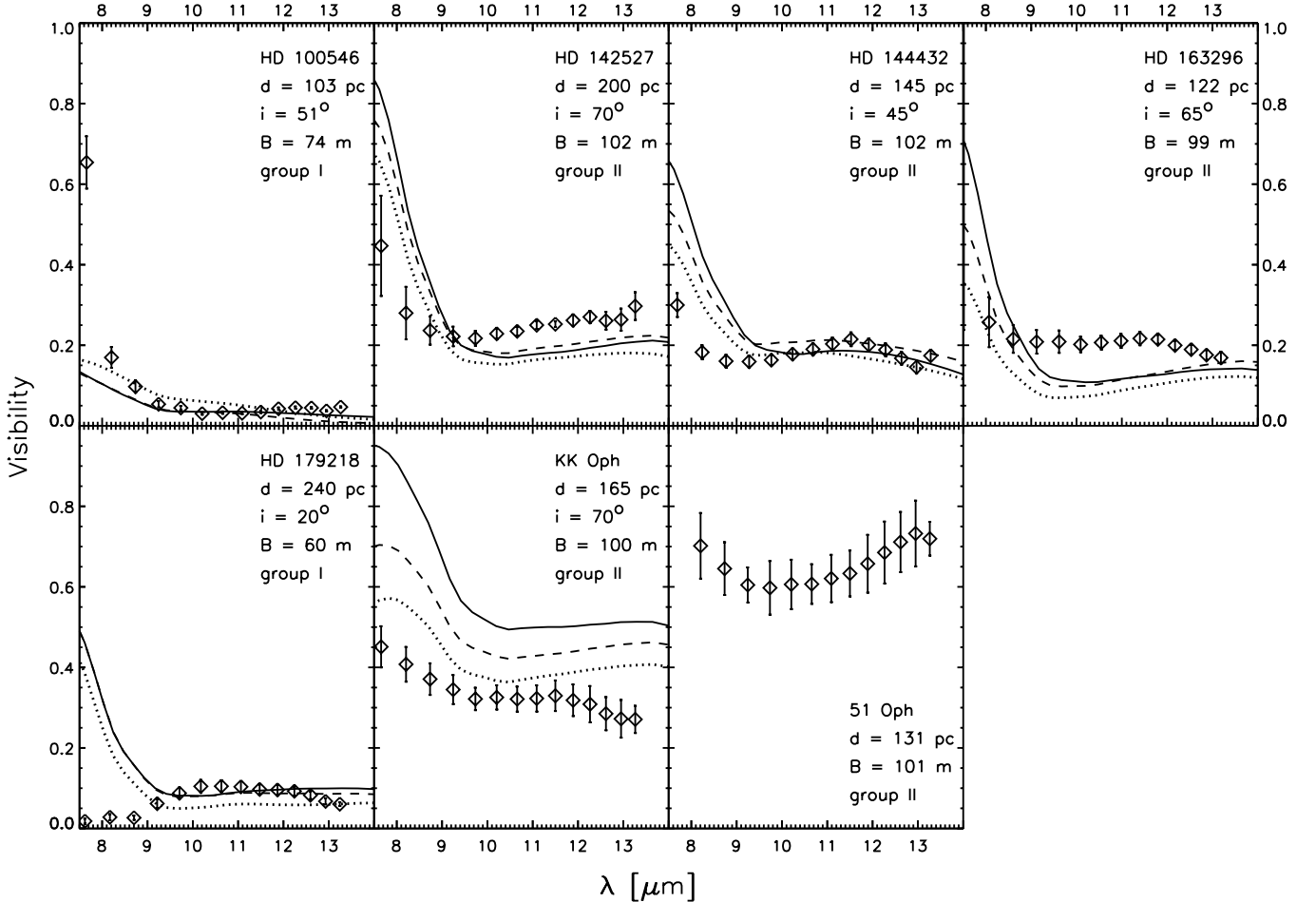
Fig. 4. The observed visibilities of the programme stars with the model predictions overplotted. These models were made with the sole purpose of fitting the spectral energy distribution and do not contain any feedback from the visibility observations. Three model visibility curves are shown: two referring to the inclination used in the SED fitting and calculated for a cut along the long axis (broken line) and along the short axis (solid line) respectively, while the dotted line is the prediction for a pole-on view. The errors give the standard deviation of the visibility results obtained for one source with different calibrators.
