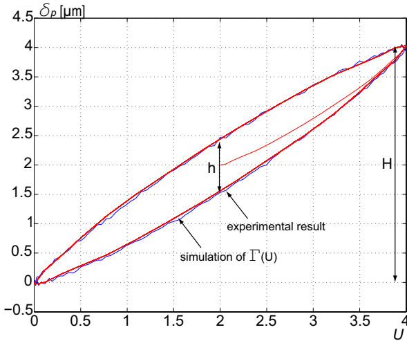
Fig. 8. Hysteresis curves: experimental result and identification result.
