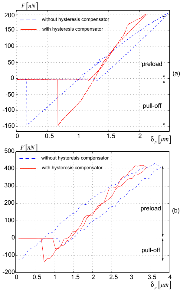
Fig. 10. Experimental result: measurement of the pull-off force between the AFM-lever and a glass substrate.
