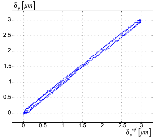
Fig. 9. Experimental result of the hysteresis compensation.
