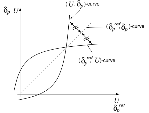
Fig. 7. Schemes showing the compensation of a hysteresis [11].
