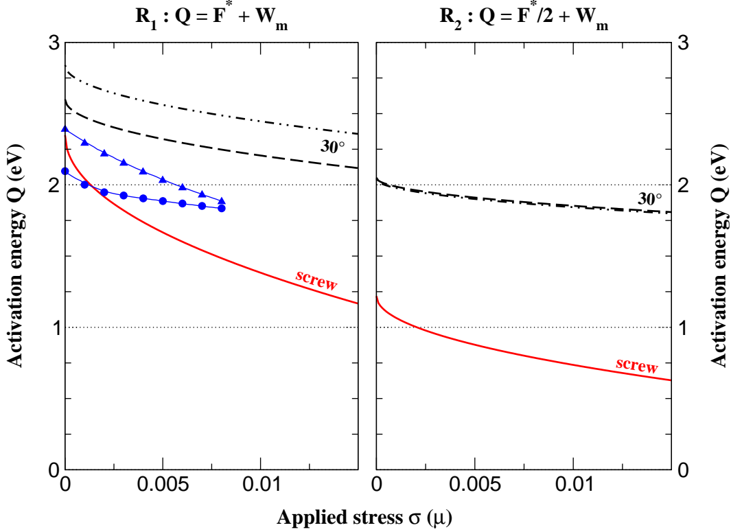
Figure 2. (color online) Activation energy for the thermally activated motion of dislocation as a function of applied stress, for Q = F^* + W_m (left panel) and Q = F^*/2 + W_m (right panel). For a 30^\circ partial dislocation, two (F_k, W_m) sets of data have been used, (0.55 eV, 1.5 eV) (dashed line) and (0.80 eV, 1.24 eV) (dot-dashed line), whereas for a shuffle screw dislocation, we have considered the computed values (1.13 eV, 0.09 eV) [22] (full line). The original data from Duesbery and Joós have also been reported (circles for the 30^\circ partial dislocation and triangles for the screw dislocation).
