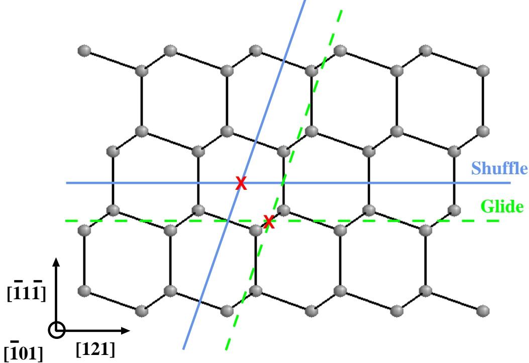
Figure 1. (color online) (101) projection of the diamond cubic structure, with the two sets of (111) planes, shuffle (full lines) and glide (dashed lines). Also shown are the two possible positions of the non-dissociated screw core.
