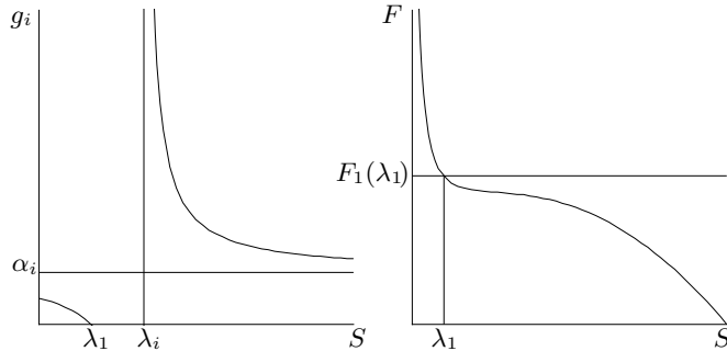
FIG. 2.1. Graphical depictions of the hypotheses 2 and 3 in Theorem 2.2. On the left, hypothesis 2. On the right, hypothesis 3.
