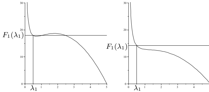
FIG. 3.2. The graph of the function F_1(S) for p_1(S) = \frac{a_1 S}{b_1 + S} (where a_1 = 2.1/1.1 , b_1 = 0.5/1.1 and \lambda_1 = 0.5 ) and y_1(S) = Y_1(1 + c_1 S) . On the left, the case c_1 = 1.8 for which hypothesis 3 in Corollary 3.1 is not satisfied. On the right, the case c_1 = 1 for which this hypothesis is satisfied.
