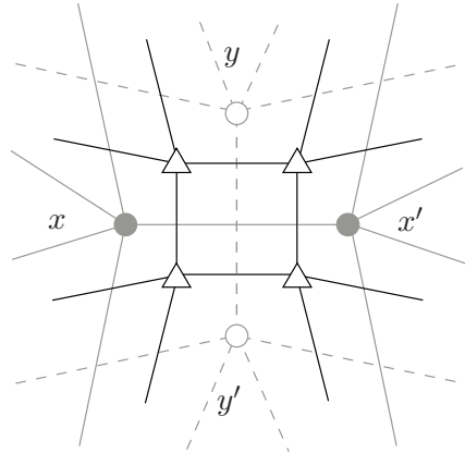
Fig. 26: The triple graph \mathcal{Y} .
