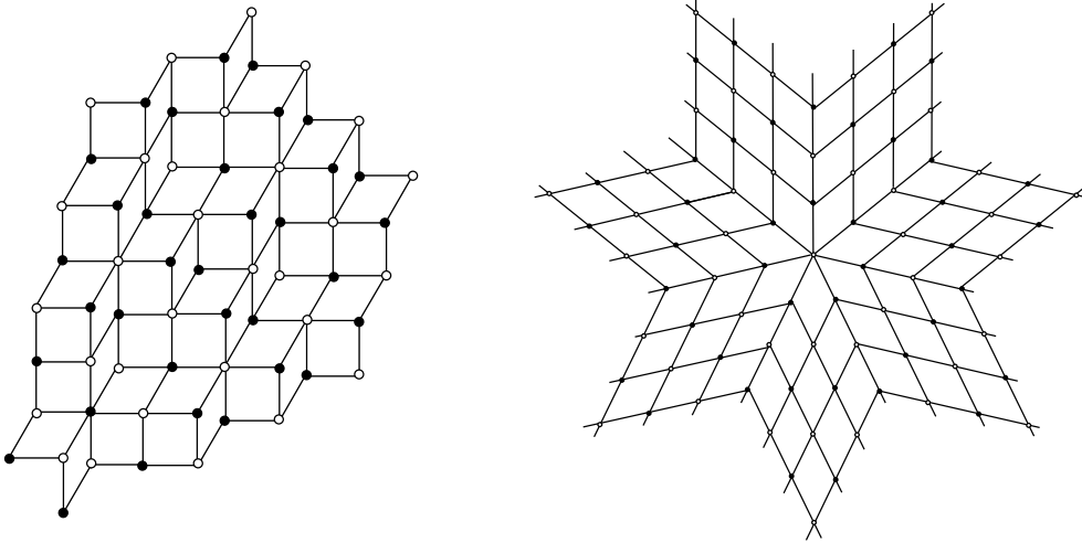
Fig. 19: Lozenge patchworks.
