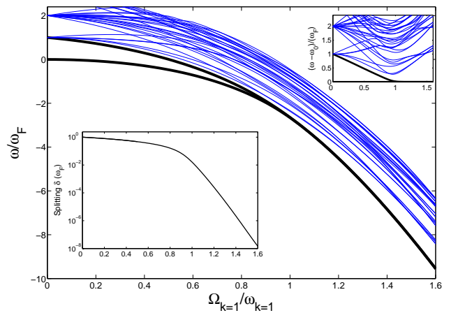
FIG. 2: First 30 energy eigenvalues (normalized to the fluxonium transition energy \hbar\omega_F ) versus dimensionless vacuum Rabi coupling for a circuit-QED system with N = 5 fluxonium atoms, N_m = 3 resonator modes (30 cut-off quanta per mode) and fluxonium frequency \omega_F = \omega_{k=1} . Due to the finite value of N , the transition from a non-degenerate to a twice degenerate ground state is not abrupt. Upper inset: the difference between the considered energy eigenvalues and the ground state energy is plotted. Lower inset: normalized energy difference (log scale) between the first 2 quasi-degenerate levels versus the dimensionless coupling. For large couplings, the two collective ground states are excellently approximated by the analytical formula in Eq. (11).
