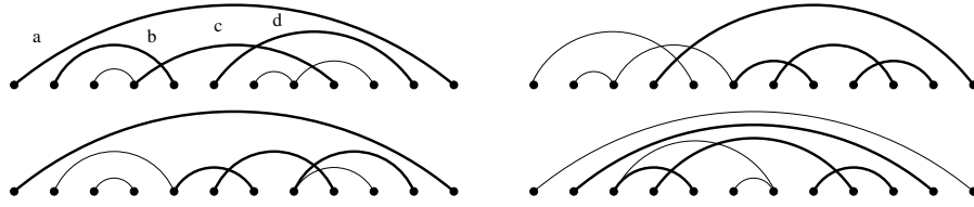
Fig. 1. Four linear graphs and a \{<, \sqsubset, \emptyset\} -common structured pattern. The occurrence of the structured pattern in each graph is emphasized in bold. Edges b, c, and d , are nesting in edge a . Edge b precedes edge d , and they both cross edge c .
