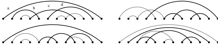
Fig. 1. Four linear graphs and a \{<, \sqsubset, \emptyset\} -common structured pattern. The occurrence of the structured pattern in each graph is emphasized in bold. Edges b, c, and d, are nesting in edge a. Edge b precedes edge d, and they both cross edge c.
