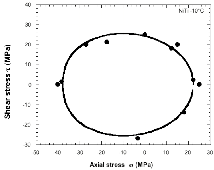
Figure 3. Tension-torsion “yield” stress surface for one way shape memory effect: theoretical (continuous line) and experimental (dots)
