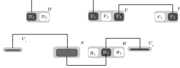
Fig. 20. Illustration of case (2). Bold lines represents sets of 2-intervals between groups.
