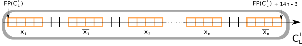
Fig. 5. Description of the simple intervals (represented as blocks of four consecutive squares) of group C_L^i .
