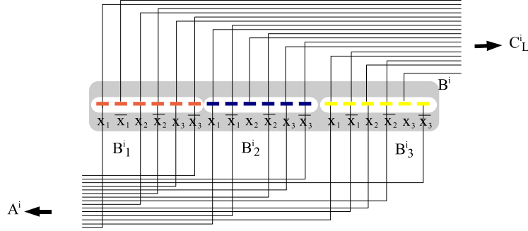
Fig. 13. Zoom on group B^i of the representation of a clause c_i = (\overline{x_1} \vee x_2 \vee x_3)
