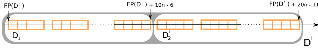
Fig. 6. Description of the simple intervals of group D^i .
