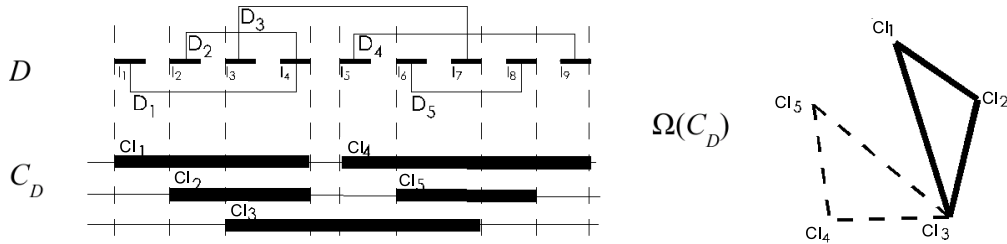
Fig. 1. Illustration of \mathcal{C}_{\mathcal{D}} and \Omega(\mathcal{C}_{\mathcal{D}}) for a given set of 2-intervals \mathcal{D} on a disjoint ground set.
