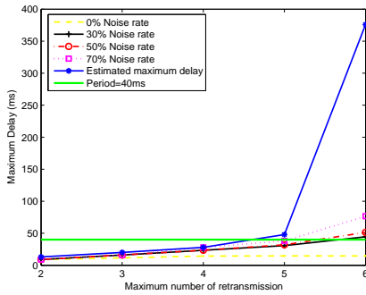
Fig. 8. Estimated/Simulated Maximum delay on charge=15%, P=40ms
