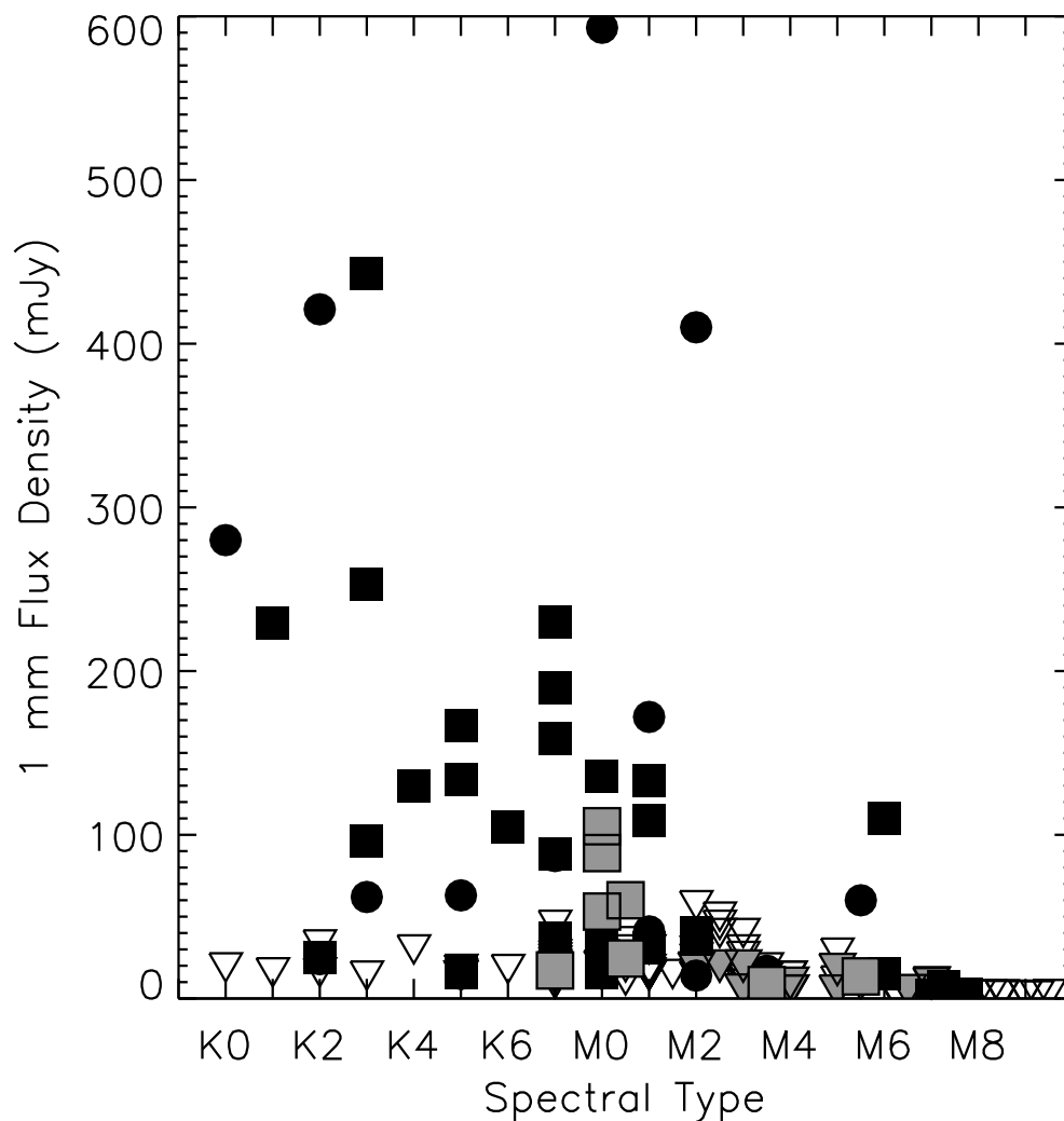
Fig. 6.— 1.3 mm flux density versus spectral type for K-M stars in the Taurus-Auriga star forming region. The sample is compiled from Beckwith et al. (1990), Osterloh & Beckwith (1995), Motte & André (2001), Scholz et al. (2006), and our sample of 23 low-mass PMS stars. The filled black squares and circles represent detections at 1.3 mm for single and binary sources, respectively, while the open triangles represent the 3\sigma upper limits. The continuum flux densities that we measured in Table 2 are represented by the large shaded symbols. There are two stars (L1551 IRS5 and HL Tau) in the K2-K5 range that have continuum fluxes larger than 800 mJy.
