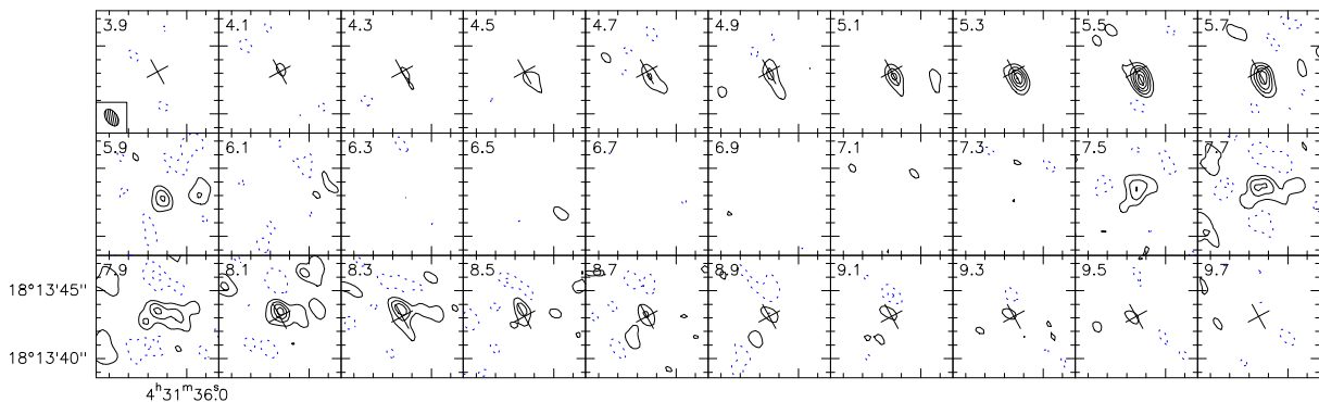
Fig. 3.— Same as Fig.1 for LkH \alpha 358. The systemic velocity is 6.80 \text{ km s}^{-1} . J=2-1 transition: resolution is 1.38 \times 0.83'' at PA 35^\circ , contour spacing 0.13 Jy, or 2.6 K ( \sim 2.9\sigma ).
