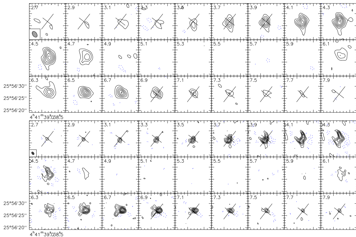
Fig. 2.— Same as Fig.1 for IRAS 04385+2550. The systemic velocity is 5.30 \text{ km s}^{-1} . Top : J=1-0 transition: resolution is 2.7 \times 1.7'' at PA 36^\circ , contour spacing 0.11 Jy, or 2.1 K ( \sim 3\sigma ). Bottom : J=2-1 transition: resolution is 1.3 \times 0.8'' , contour spacing 0.13 Jy, or 2.8 K ( \sim 3\sigma ).
