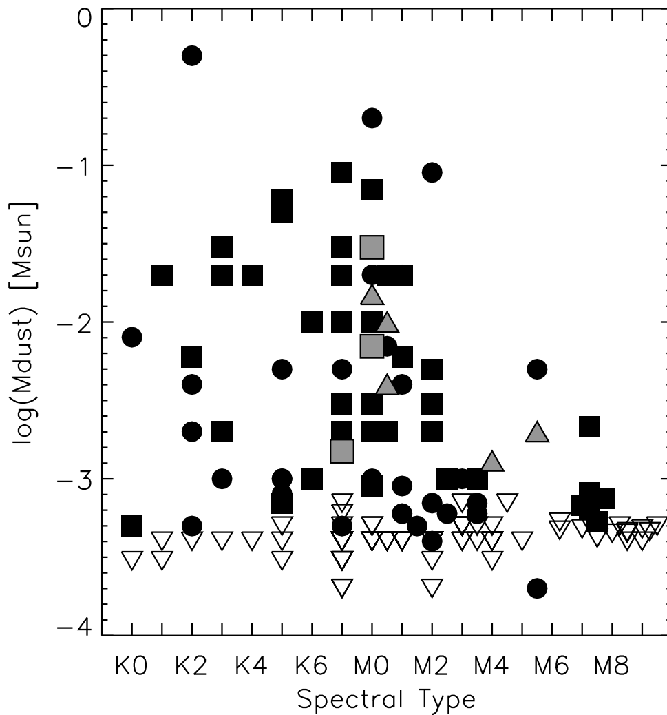
Fig. 8.— Dust disk masses versus spectral type for K-M stars in the Taurus-Auriga star forming region. The filled black squares and circles represent the dust masses determined by Andrews & Williams (2005) and Scholz et al. (2006) for single and binary sources, respectively, while the open downward pointing triangles represent their 3\sigma upper limits. Our dust disk mass measurements listed in Table 4 are represented by the large shaded squares while the shaded upward pointing triangles represent our lower limits.
