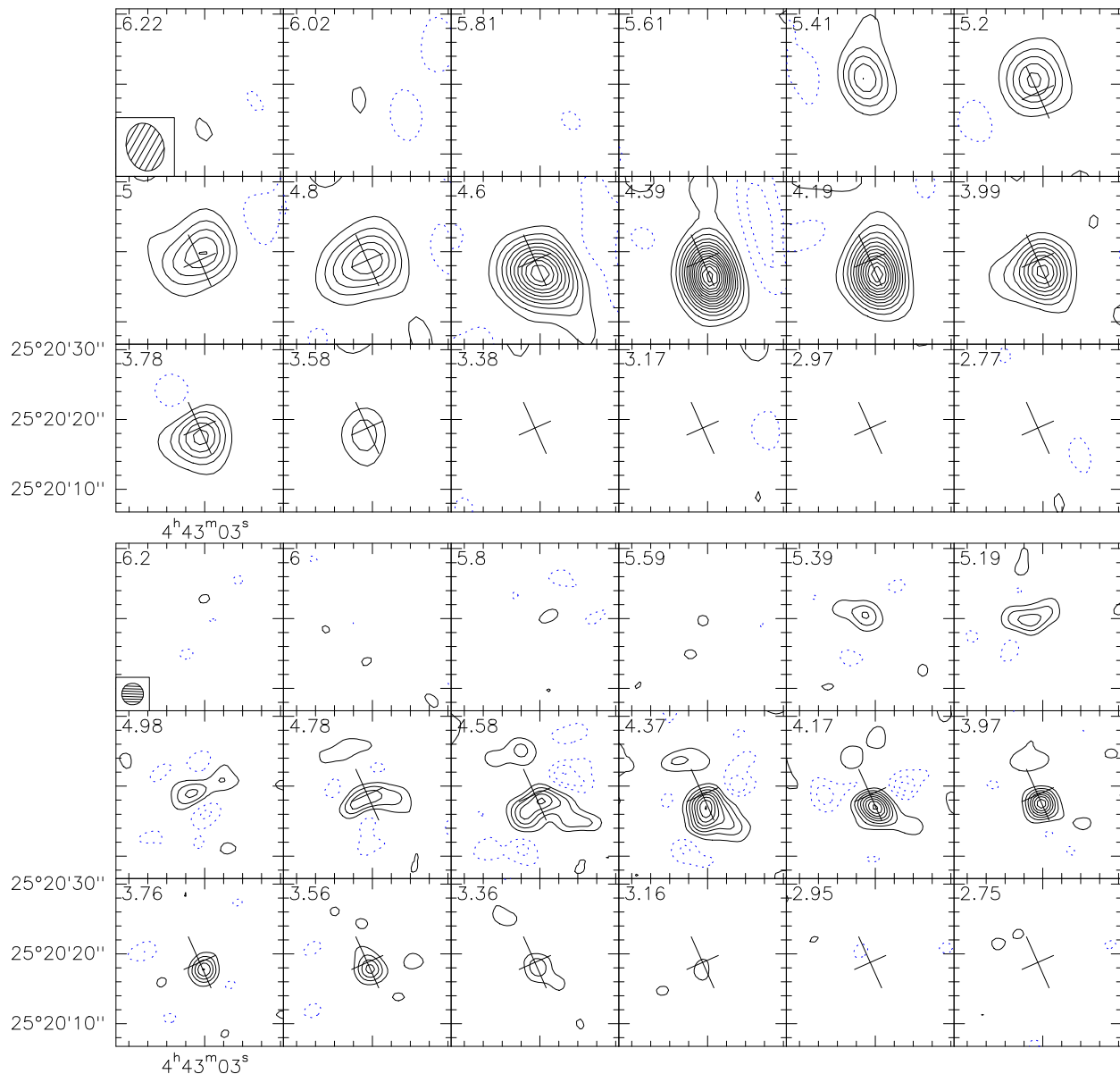
Fig. 1.— ^{12}\text{CO} J=1-0 and J=2-1 maps for GO Tau, with LSR velocity indicated in each panel. The systemic velocity is 5.0 \text{ km s}^{-1} . The crosses indicate the disk orientation and center position; channels with no crosses have not been used in the analysis of the rotating disk. Top : J=1-0 transition: resolution is 6.9 \times 5.4'' at PA 15^\circ , contour spacing 0.1 Jy, or 0.25 K ( \sim 2.5\sigma ). Bottom : J=2-1 transition: resolution is 3.1'' , contour spacing 0.3 Jy, or 0.7 K ( \sim 2.5\sigma ).
