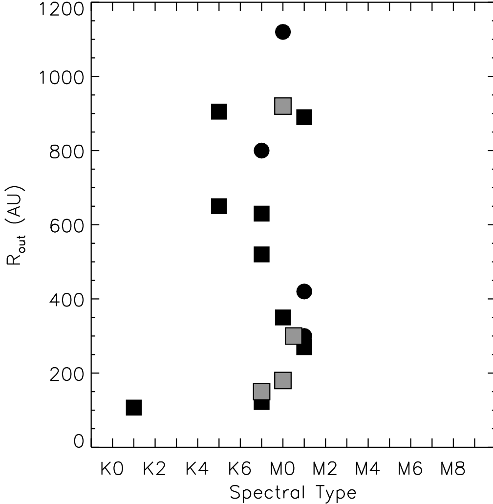
Fig. 5.— Radii of CO disks detected around T Tauri stars of spectral types K-M in the Taurus-Auriga star forming region. The large shaded squares represent our measurements of R_{\text{out}} for LkH \alpha 358, GO Tau, Haro 6-13, and IRAS 04385+2550. The solid black squares represent values of R_{\text{out}} measured for the single stars CY Tau, DL Tau (Simon et al. 2000), BP Tau (Dutrey et al. 2003), DM Tau, LkCa 15 (Piétu et al. 2007), and GM Aur (Dutrey et al. 2008), and the radius at half-maximum measured for DO Tau, RY Tau (Koerner & Sargent 1995), and Haro 6-5B (Yokogawa et al. 2002). The solid black circles represent the radii of the circumbinary disks around GG Tau A (Dutrey et al. 1994), UY Aur (Duvert et al. 1998), UZ Tau E (Simon et al. 2000), and HH 30 (Pety et al. 2006; Guilloteau et al. 2008).
