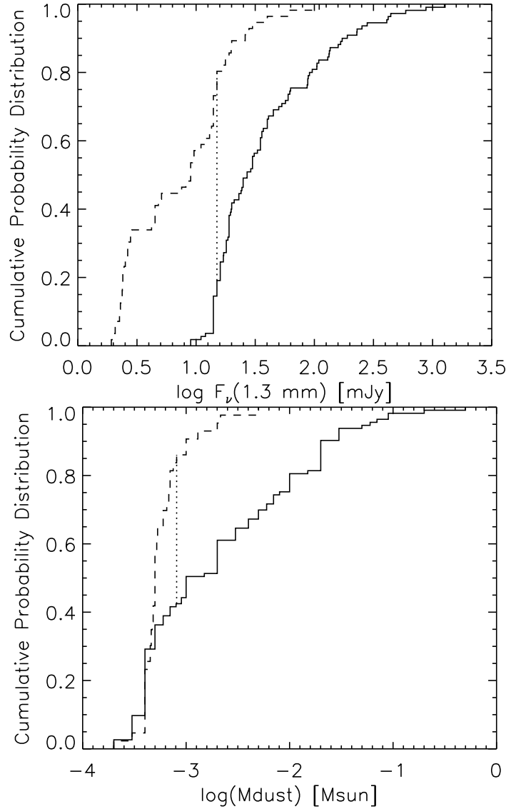
Fig. 7.— Top : Cumulative probability function for 1.3 mm continuum flux densities. The solid line represents the sample of T Tauri stars with spectral types between K0-M2, while the dashed line represents the sample between M3-M9. The maximum difference between the distributions of 0.61 (dotted line, Kolmogorov-Smirnov statistic) indicates that the distributions are significantly different. Bottom : Cumulative probability function for the values of M_{\text{dust}} . The samples are defined in the same way as the top panel. The maximum difference between the distributions of 0.44 indicates that the distributions are significantly different. In both cases, the Kolmogorov-Smirnov test indicates a negligible probability ( p \ll 0.01 ) that the two distributions are actually the same.
