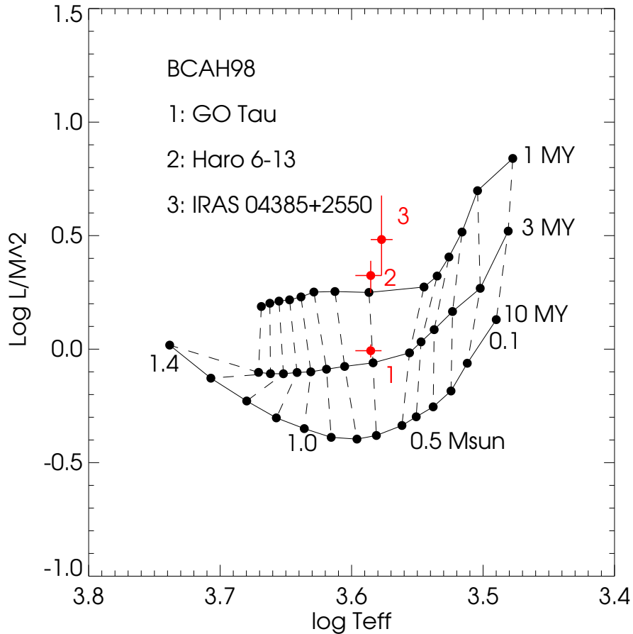
Fig. 9.— Evolutionary tracks computed by Baraffe et al. (1998) plotted as the distance independent quantity L/M^2 versus T_{\text{eff}} . The tracks are plotted from 0.1-1.4 M_{\odot} at intervals 0.1 M_{\odot} for an age range of 1-10 Myr. We show the location of GO Tau, Haro 6-13, and IRAS 04385+2550 (red circles) using the L_{\text{star}} values (Table 1, Column 5) computed by White & Ghez (2001) and White & Hillenbrand (2004), T_{\text{eff}} from Table 1, and the dynamical masses derived from the CO emission (Table 5). We propagated the dynamical mass uncertainties through to the L/M^2 values and assumed \pm 0.5 spectral subtype uncertainties on T_{\text{eff}} .
