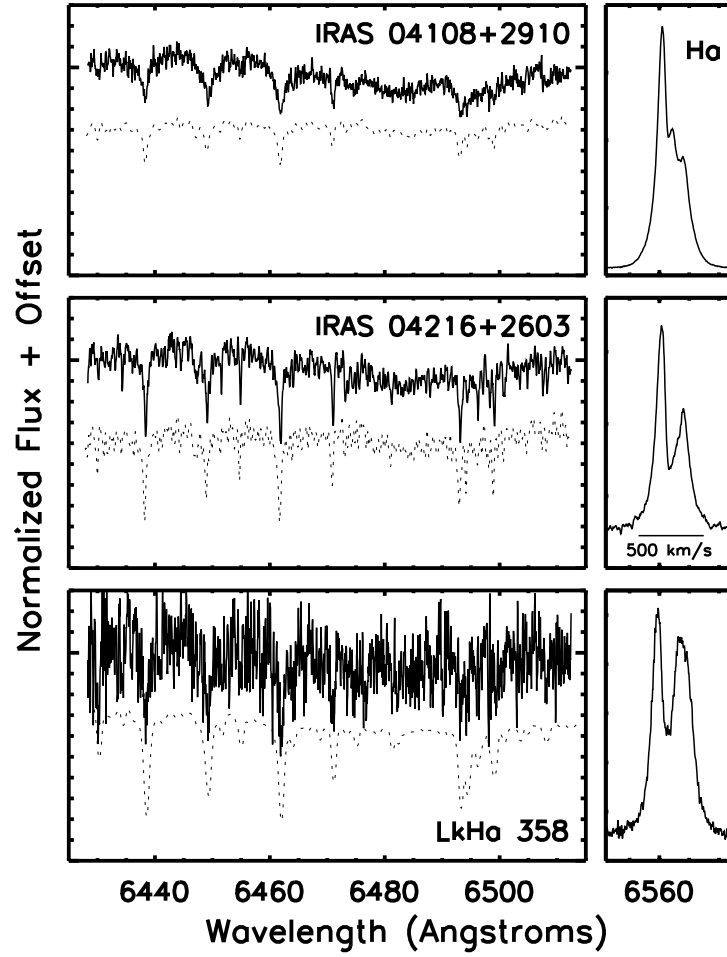
Fig. 10.— Portions of the Keck/HIRES spectra within the R band (left) and H \alpha emission profiles (right); both panels have the same wavelength scale. The best-fit dwarf standards, rotationally broadened and optically veiled, are shown as dashed lines for comparison. The strong, broad H \alpha emission profiles suggest that all three stars are accreting.
