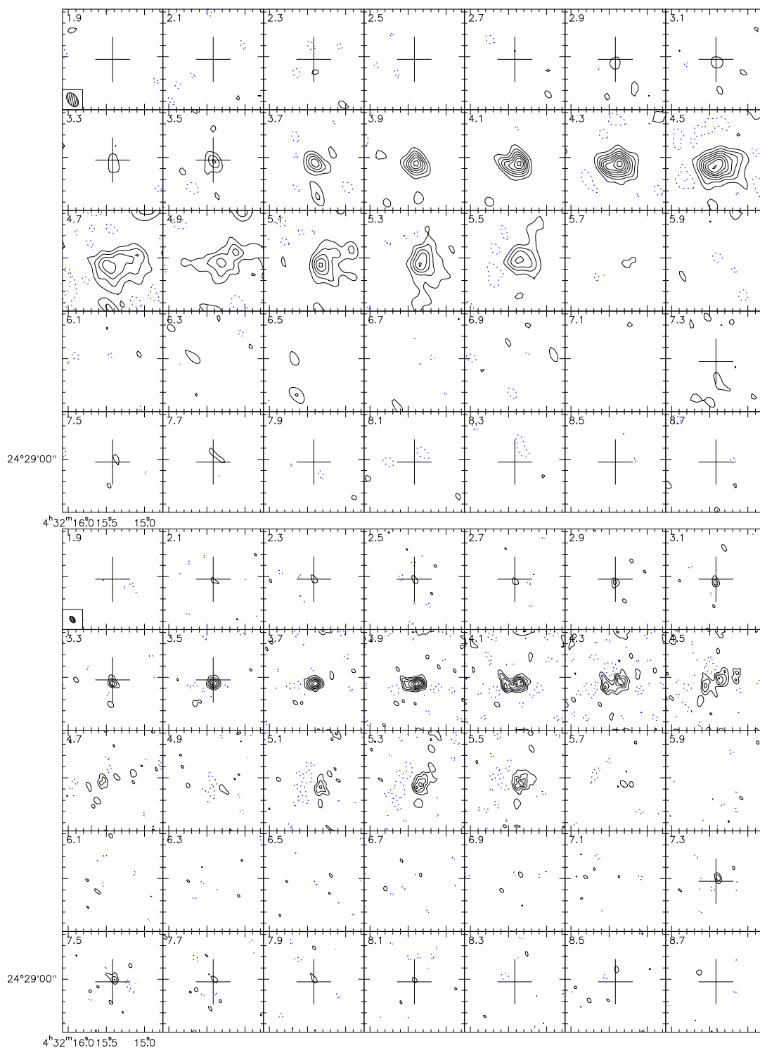
Fig. 4.— Same as Fig.1 for Haro 6-13. The systemic velocity is 5.10 \text{ km s}^{-1} . Top : J=1-0 transition: resolution is 2.8 \times 2.7'' at PA 34^\circ , contour spacing 0.10 \text{ Jy} , or 1.9 \text{ K} ( \sim 2.8\sigma ). Bottom : J=2-1 transition: resolution is 1.35 \times 0.80'' at PA 37^\circ , contour spacing 0.13 \text{ Jy} , or 2.8 \text{ K} ( \sim 2.8\sigma ).
