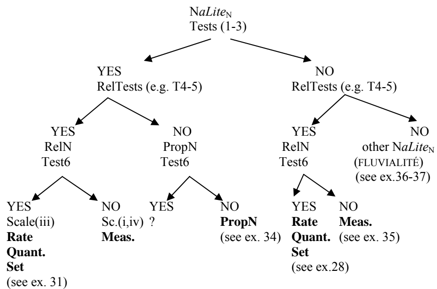
Figure 4. NaLite N interpretation: Decision tree.
