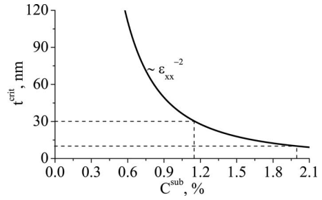
FIG. 2. Critical layer thickness t^{\text{crit}} as a function of C^{\text{sub}} in s -Si:C layers.
