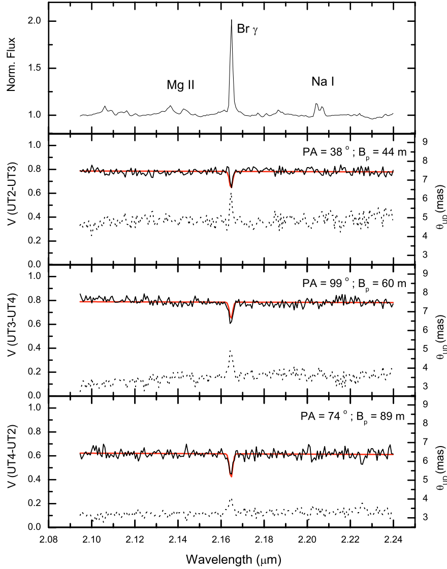
Fig. 2. AMBER/VLTI observations of CPD–57° 2874 obtained around Br \gamma with spectral resolution R = 1500 . The normalized flux is shown in the top panel and the visibilities V for each baseline (30% best frames) are given in the other panels (the corresponding projected baselines B_p and position angles PA are indicated). The errors in V are \approx \pm 5\% . The dotted lines are the uniform disk angular diameters \theta_{UD} (to be read from the scales on the right axis), computed from V at each \lambda as a zero-order size estimate. The visibilities obtained from the elliptical Gaussian model fit the observations quite well (smooth solid lines; Eqs. (1) and (2), and Table 4). In contrast to the Br \gamma line, the Mg II and Na I lines do not show any clear signature in the visibilities.
