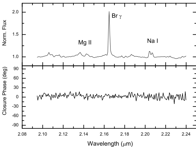
Fig. 4. AMBER/VLTI closure phase for CPD–57° 2874 obtained around \text{Br}\gamma with spectral resolution R = 1500 . Within the noise level ( \approx \pm 10^\circ ) the closure phase is zero both in the continuum and in the \text{Br}\gamma line. This strongly suggests that the CSE has an approximately centrally-symmetric projected intensity distribution in the near-IR.
