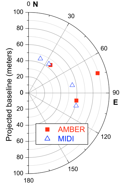
Fig. 1. Projected baselines and corresponding position angles for the AMBER and MIDI observations of CPD-57° 2874 (see also Table 1).
