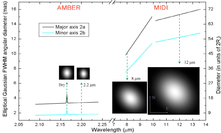
Fig. 5. Size and orientation of the CSE derived from the fit of an elliptical Gaussian model (Eqs. (1) and (2)) to the AMBER/VLTI and MIDI/VLTI visibilities (the corresponding fit parameters are listed in Table 4). The scale in the right is given in stellar diameters ( 2R_* ), where the radius R_* is estimated to be 60 \pm 15 R_\odot (Sect. 3).
