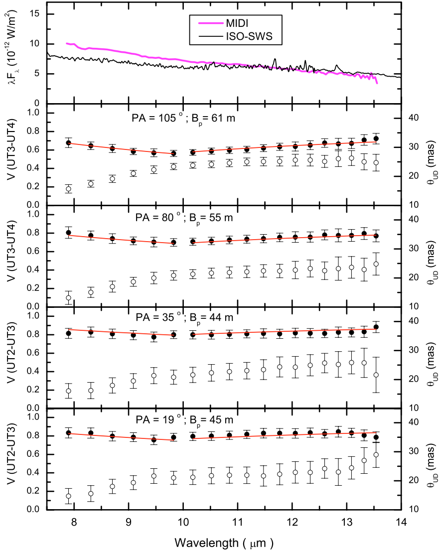
Fig. 3. MIDI/VLTI observations of CPD–57° 2874 obtained in the mid-IR with spectral resolution R = 30 . This figure is organized as Fig. 2, but here V and \theta_{UD} are shown as filled and open circles, respectively. The MIDI and ISO-SWS (Sloan et al. 2003) spectra ( top panel ) do not show any clear evidence of a silicate feature around 10\ \mu\text{m} . The MIDI visibilities are well fitted with an elliptical Gaussian model (solid lines; Eqs. (1) and (2), and Table 4).
