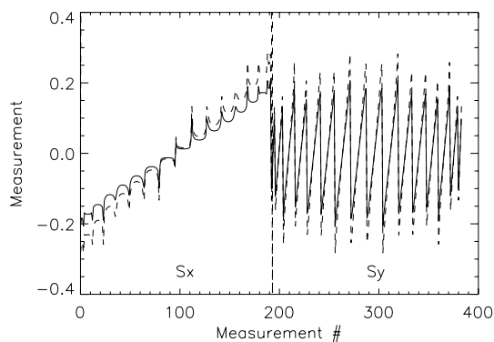
Figure 5. Measurements vector due to interference for a null incoming phase for a centre-to-centre pupil separation of 1.3. Solid line, PSF sampling = 32; dashed line, PSF sampling = 4.
