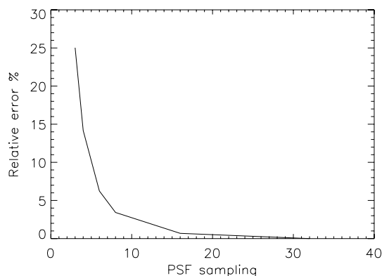
Figure 6. Error on the null measurements in function of the PSF sampling parameter. The reference measurement used to estimate the error has been computed for a PSF sampling value of 32.
