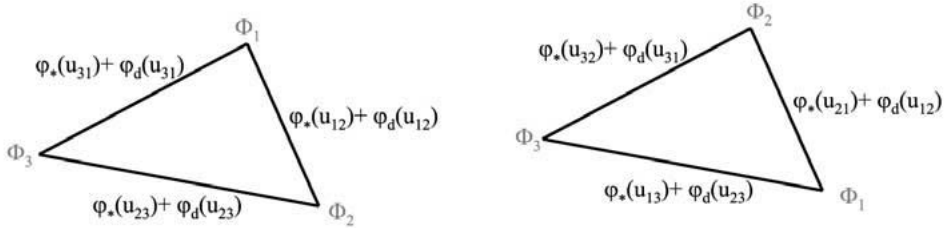
Figure 2. Closure phase before and after beam commutation.
