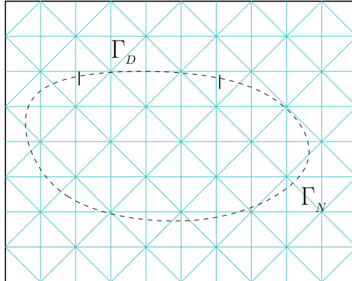
FIGURE 3.1. Example of a structured mesh.
