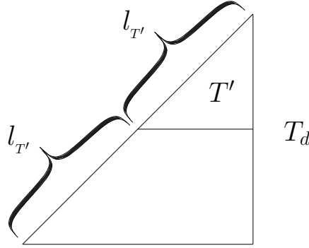
FIGURE 5.2. Prolongation of T' .
