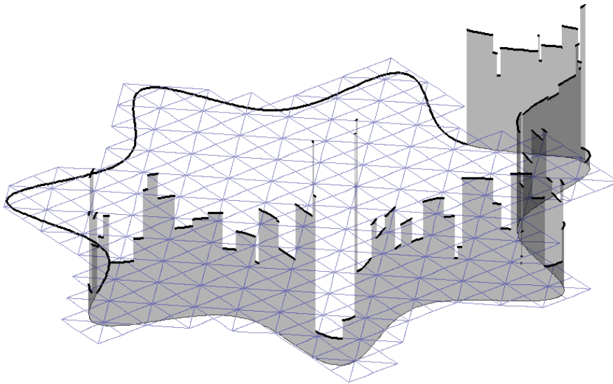
FIGURE 7.5. Multiplier on \Gamma_D with the Barbosa-Hughes stabilization for the P_1/P_0 method ( h = 0.05 ).
