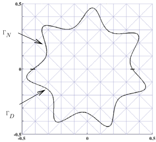
FIGURE 6.1. Test domain and a triangular structured mesh.
