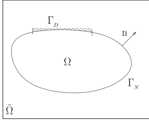
FIGURE 2.1. Fictitious and real domains.
