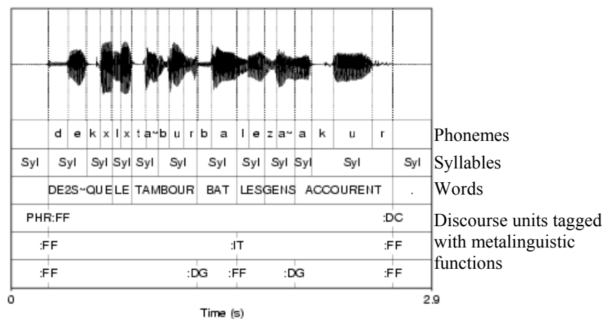
Figure 2: A speech sample ('As soon as the drum starts, the people rush.') for the SFC, labeled using Praat. The [:FF] tag delimits the beginning and end of units. Other tags are used to label the metalinguistic functions [:DC] for declarative sentence, [:IT] between clauses, [:DG] between nominal and verbal groups.
