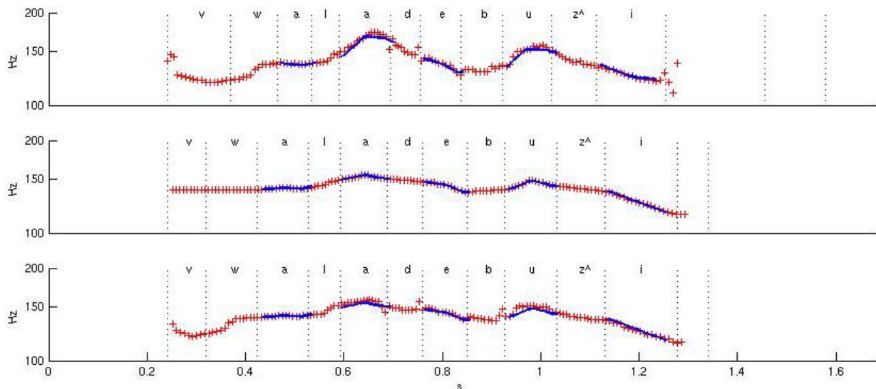
Figure 3: Illustration of giving flesh to the melodic skeleton of a French utterance ( Voilà, des bougies ! 'Look -- candles!'). Top: original f_0 curve with stylization superposed. Middle: melodic skeleton predicted by the SFC model trained using 235 such utterances (first training loop). Bottom: final predicted f_0 curve with melodic skeleton also superposed. Microprosodic details such as bursts in plosives (/d/ and /b/ here) or f_0 dips in the initial /v/ are reproduced by adding deviations between original f_0 curve and stylization to the predicted melodic skeleton (displayed in the top panel).
