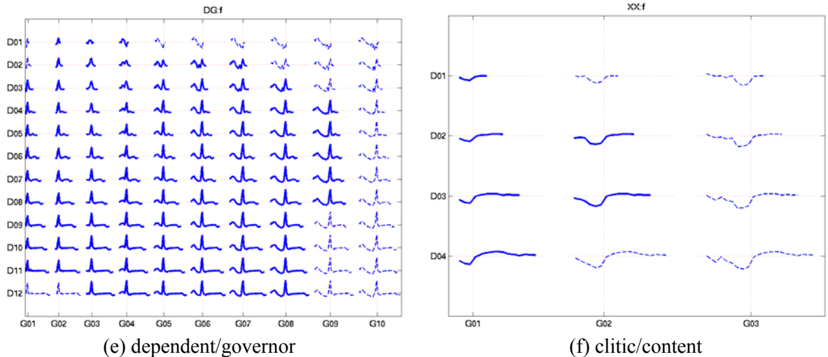
Figure 5. Expansion of f_0 movement for different metalinguistic functions applied to units with increasing size. These expansions are synthesized by trained contour generators. Contours with dotted lines are extrapolated, i.e. no exemplars are present in the training corpus. Top: modalities and prosodic attitudes in French: (a) assertion, (b) question, (c) incredulous question, (d) statement of an obvious fact. Please note that contour generators learn the laws governing the variation of the global slope of the contours and final movements of that contours thanks to the absolute and relative linear ramps (see Figure 4): the relationship between global slope and amplitude of the final melodic movement versus sentence length may be nonlinear. Bottom: linking two constituents (abscissa/ordinate: size of first/second unit): (e) between a governor and its left dependent when considering a dependency tree (see §1.1) (f) between a clitic word and the following content word (e.g. f_0 dip on the determiner preceding a noun).
