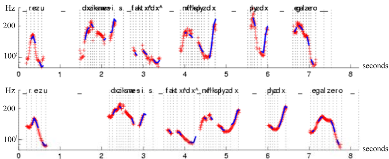
Figure 10: Comparing original and predicted F0 contours for the same formula as Figure 8. Top Original and stylized f0 curve. Bottom: stylized f0 curve predicted by the SFC.
