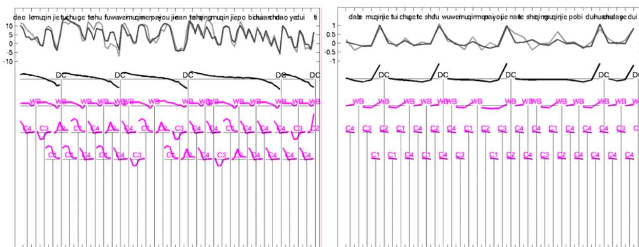
Figure 11: Decomposing the melodic (left) and rhythmic (right) contours of a recording consisting of five Chinese sentences. Same conventions as for Figure 7. In each subfigure, from top to bottom: superposition of original (light gray) and predicted (dark gray) prosodic skeleton; sentence-specific contours; word-specific contours and tone-specific contours. The tone contours are displayed in two rows for sake of clarity since they overlap. The scope of each tone contour is two syllables: the syllable carrying the tone and the following one (except for the last syllable of each sentence, where only the tone-bearing syllable is considered). No group- or clause-specific contours have been yet introduced.
