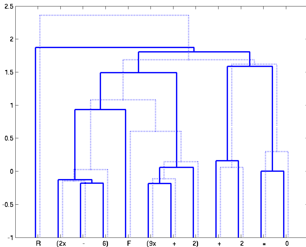
Figure 9: Performance structures (Gee and Grosjean 1983) of the original (plain) and predicted (dotted) prosody for the same formula as Figure 8. We use here lengthening factors of the last syllable of each word as a cue for word grouping. We provide here a more structural view of the data already displayed in Figure 8.b. One can see that the SFC renders properly the hierarchy except the balance between the first two operands of the formula.
