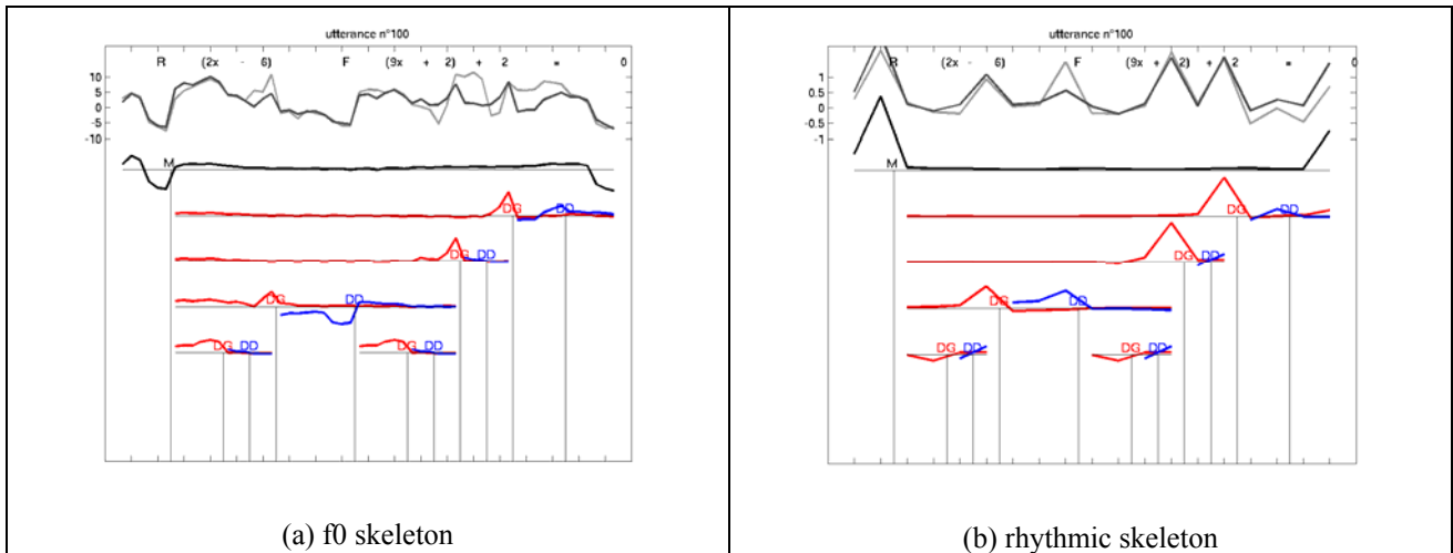
Figure 8: Analyzing and predicting the prosodic skeleton of a spoken mathematical formula (“solve: (2x-6)x(9x+2)+2=0 ”). The f_0 skeleton is figured on the left hand side using the same conventions as for Figure 7. The rhythmic skeleton is figured on the right hand side using also the same conventions except that the lengthening factor is displayed per syllable instead of three f_0 values. Three discourse functions are here recruited (M, DG and DD) and applied to different scopes in order to encode the hierarchical syntactic relations between the different terms of the formula. The SFC has been trained on 132 such spoken maths.
