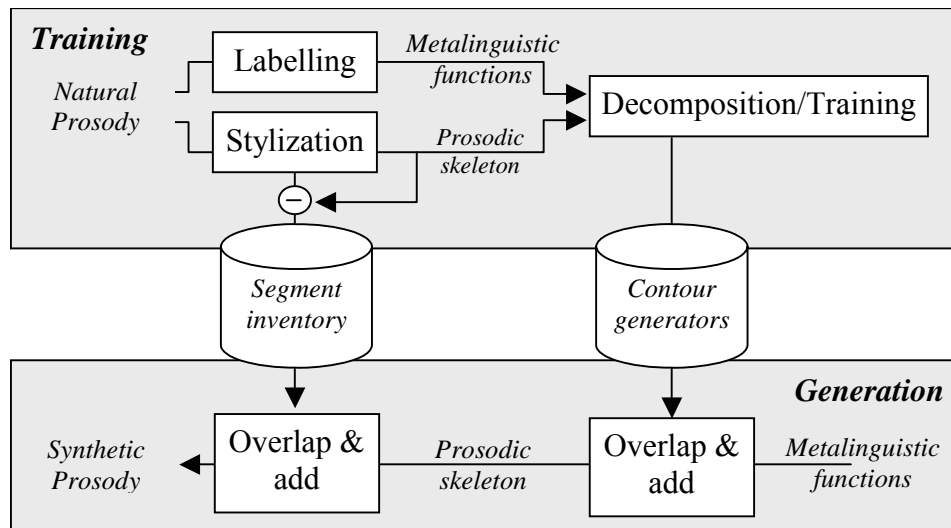
Figure 1: Training the SFC consists in decomposing prosodic skeletons (stylized prosodic contours) of a set of training utterances into overlapping multiparametric elementary contours associated with the metalinguistic functions they recruit. One contour generator is responsible for generating multiparametric elementary contours associated with one metalinguistic function given its scope (the phonological units the function is applied to). The prosodic flesh obtained by subtracting the prosodic skeleton to the original prosody is stored into the characteristics of the acoustic segments used by the concatenative speech synthesizer. The generation process consists simply in the selection of the appropriate contour generators implementing the various metalinguistic functions recruited by the discourse and overlap-and-add them with the prosodic flesh of the segments used. Note that the generation process is also used during the training phase for decomposing prosodic skeletons into multiparametric elementary contours (see Figure 6 and section 3.2).
