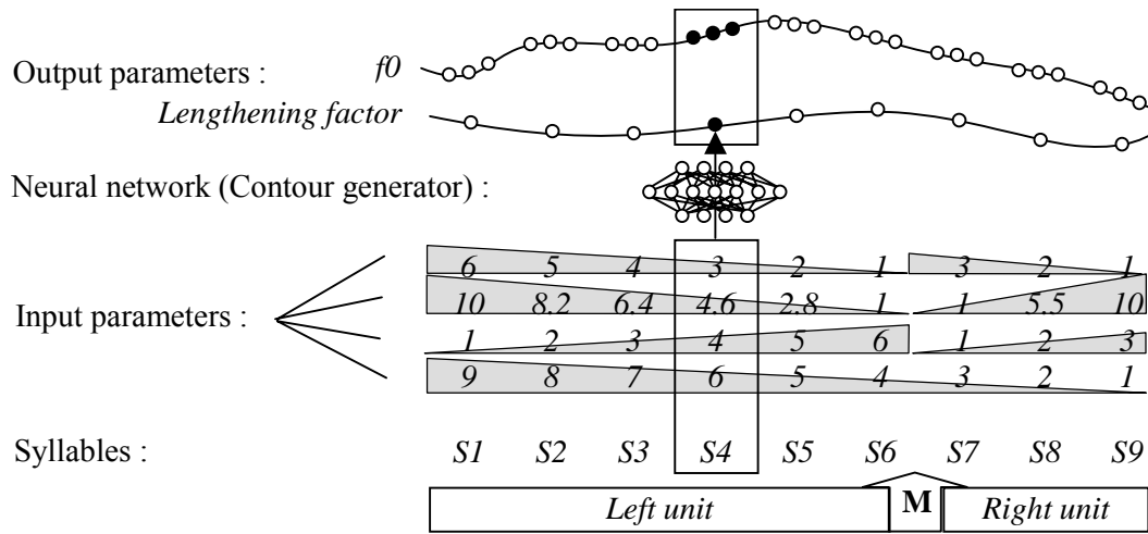
Figure 4: Example of the implementation of a function M by a contour generator on two units of respectively six and three syllables. The generator computes four output parameters per syllable (three f_0 values and a lengthening factor; see §2). Each syllable is characterized by four input parameters that specify the relative and absolute position of that syllable within the scope. The input parameters are thus series of linear ramps varying between the extreme values 1 and 10. From bottom to top: relative distance to the end of the scope; relative and absolute distance to the beginning/end of the unit to which it belongs.
