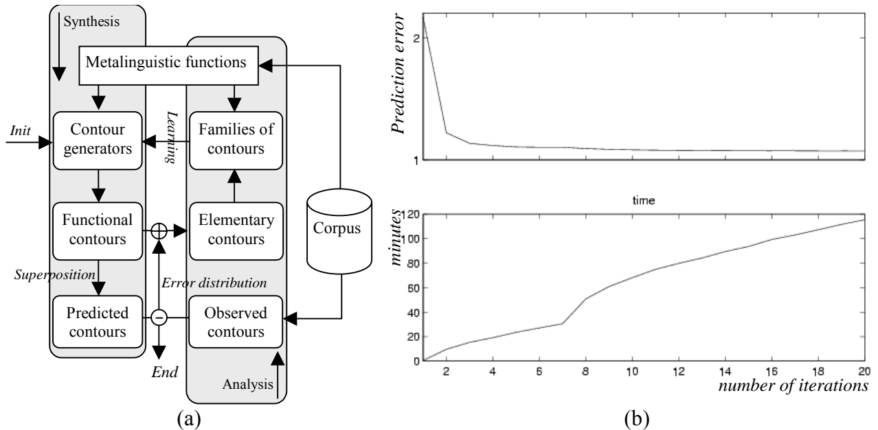
Figure 6: (a) Analysis-by-synthesis loop. SFC generators are trained using patterns built by adding to what they already predict a proportion of what they together still do not predict, i.e. the difference between observed and predicted contours at the iteration considered (see §3.2 for detailed comments on the training loop). The learning loop stops when this difference no longer diminishes significantly. (b) Typical evolution of the reconstruction error (top) and training time on a standard Pentium III computer (bottom) for a sample corpus (1,000 utterances; 6 contour generators) as a function of the number of iterations. Convergence is obtained within a few dozen iterations.
