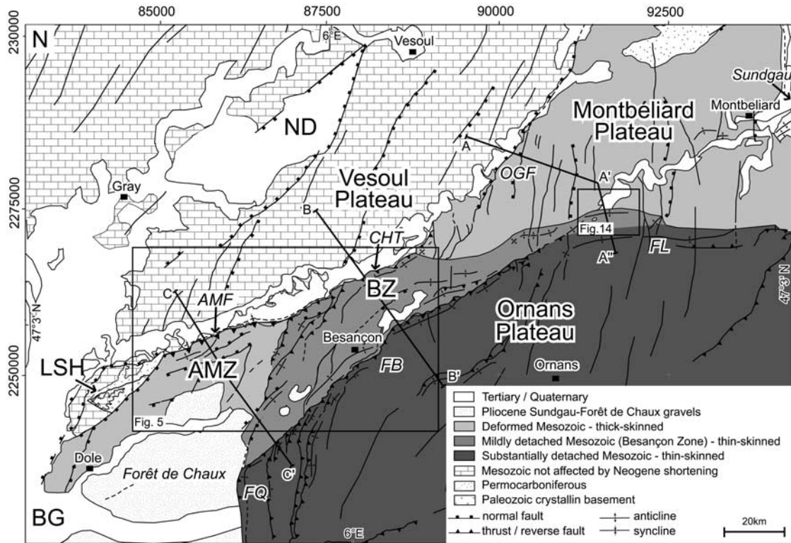
Figure 3. Tectonic map of the study area, showing the new subdivision based on the results of this study (see text for discussion). Note the traces of three cross sections shown in Figure 8. AMF, Avant-Monts Fault; AMZ, Avant-Monts Zone; BZ, Besançon Zone; BG, Bresse Graben; CHT, Chailluz Thrust; FB, Faisceau Bisontin; FL, Faisceau du Lomont; FQ, Faisceau de Quingey; LSH, La Serre Horst; ND, Noidans Basin; OGF, Ognon Fault.
